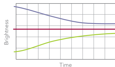
— Constant regulated brightness — Natural lamp brightness — Lamp power
